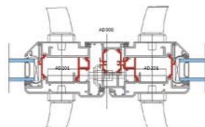
Interlock Detail
