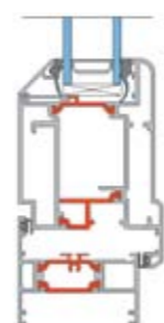
Cill Detail
